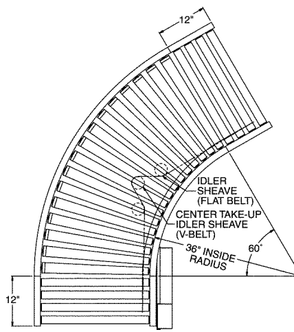
60° CURVE
